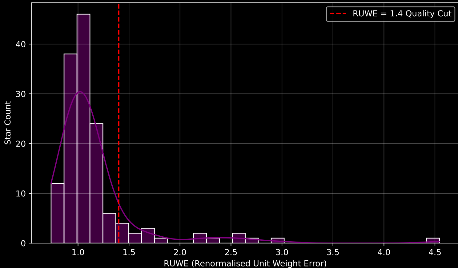
GAPOGEE DR17 Field [280-38-O_TESS] RUWE Distribution (n= 144)
