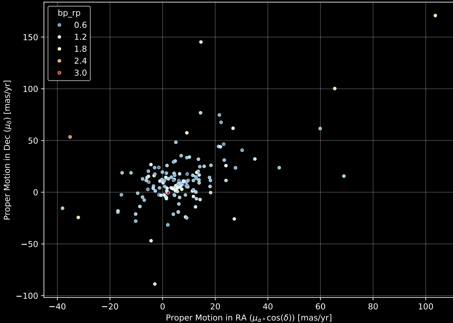
APOGEE DR17 Field: [280-38-O_TESS] Proper Motion Diagram (n= 153)
