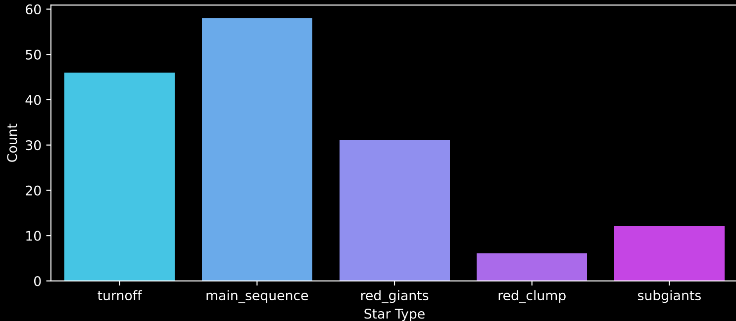
APOGEE DR17 Field: [280-38-O_TESS] Count plot of Star Type
