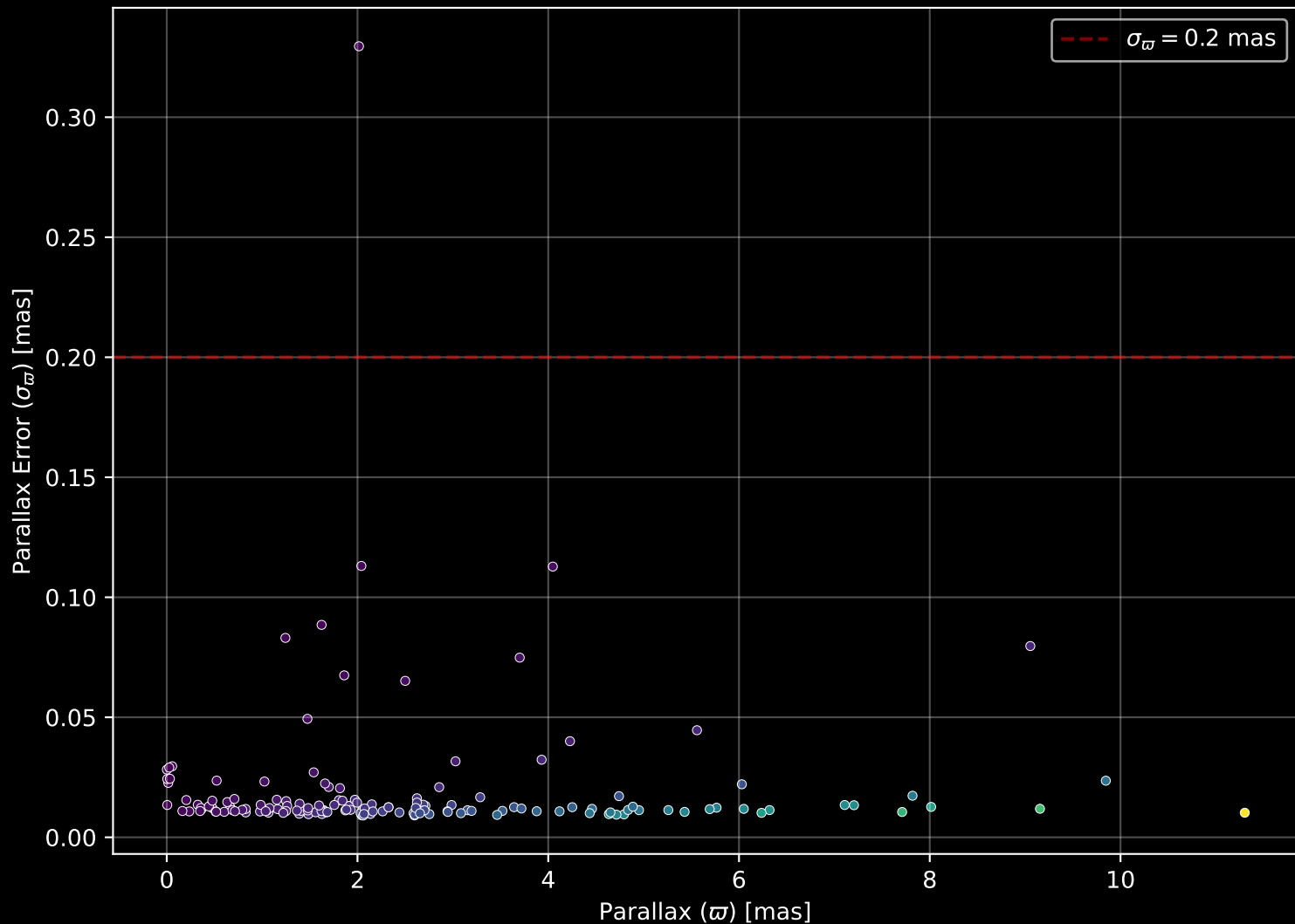
APOGEE DR17 Field: [280-38-O_TESS] Parallax Quality (n= 153)
