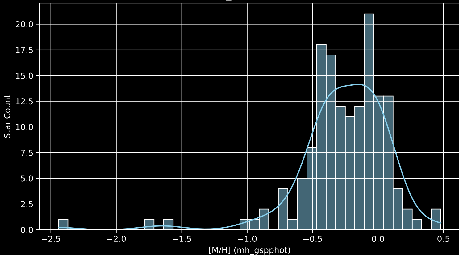
APOGEE DR17 Field: [280-38-O_TESS [M/H] (mh_gspphot) (n= 151)
